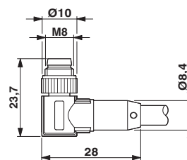
Dimensional drawing
