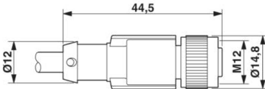
Dimensional drawing
