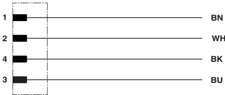
Contact assignment of the M12 plug
