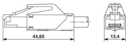
Dimensional drawing
