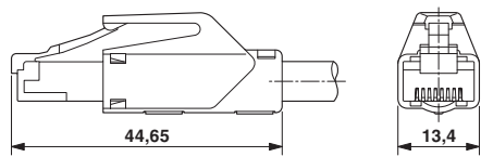
Dimensional drawing
