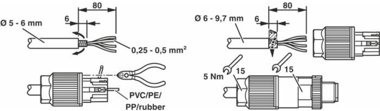
Functional drawing
