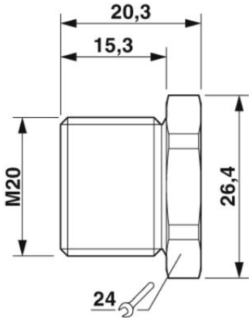
Dimensional drawing
