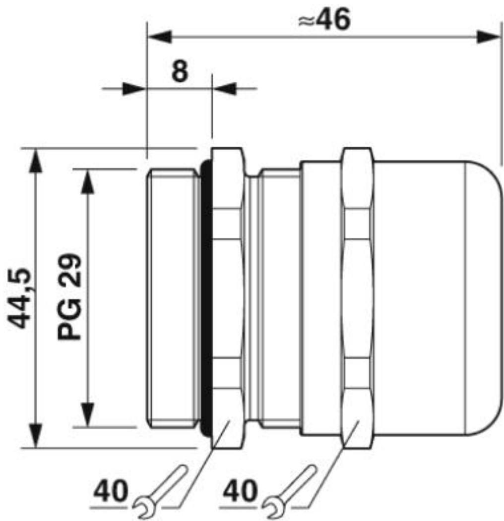
Dimensional drawing
