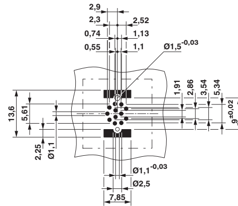
Drilling diagram
