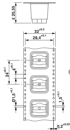
Dimensional drawing
