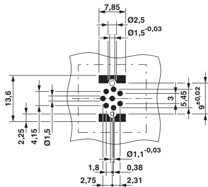
Drilling diagram
