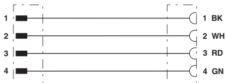
Contact assignment of 7/8" plugs/sockets
