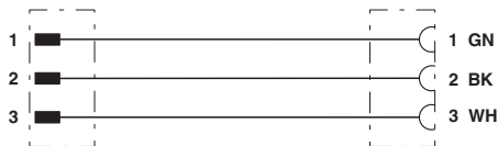
Contact assignment of 7/8" plugs/sockets
