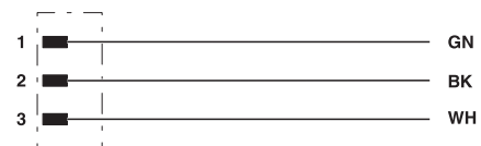
Contact assignment of the 7/8" plug
