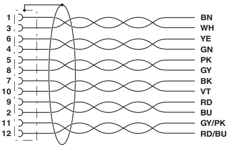
Contact assignment of the M12 socket
