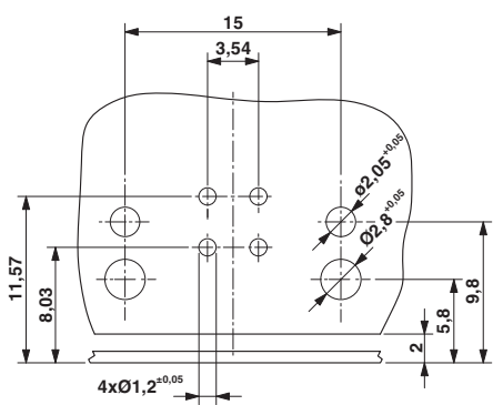
Drilling diagram
