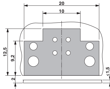
Dimensional drawing
