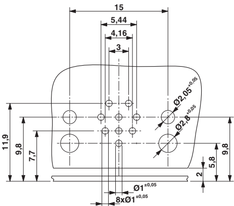
Drilling diagram
