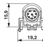
M12 flush-type connector, socket, contact carrier, front view
