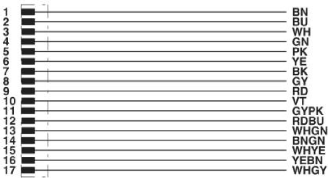
Contact assignment of the M12 plugs
