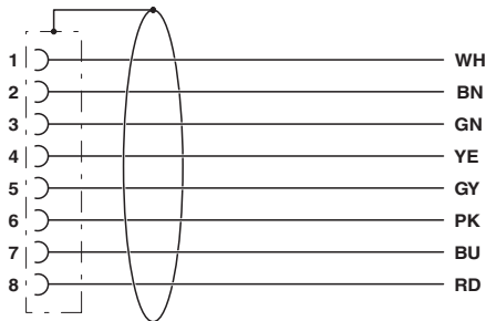
Circuit diagram
