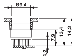
Dimensional drawing
