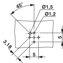
Drilling diagram
