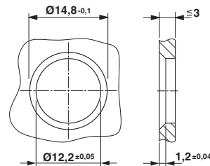
Dimensional drawing
