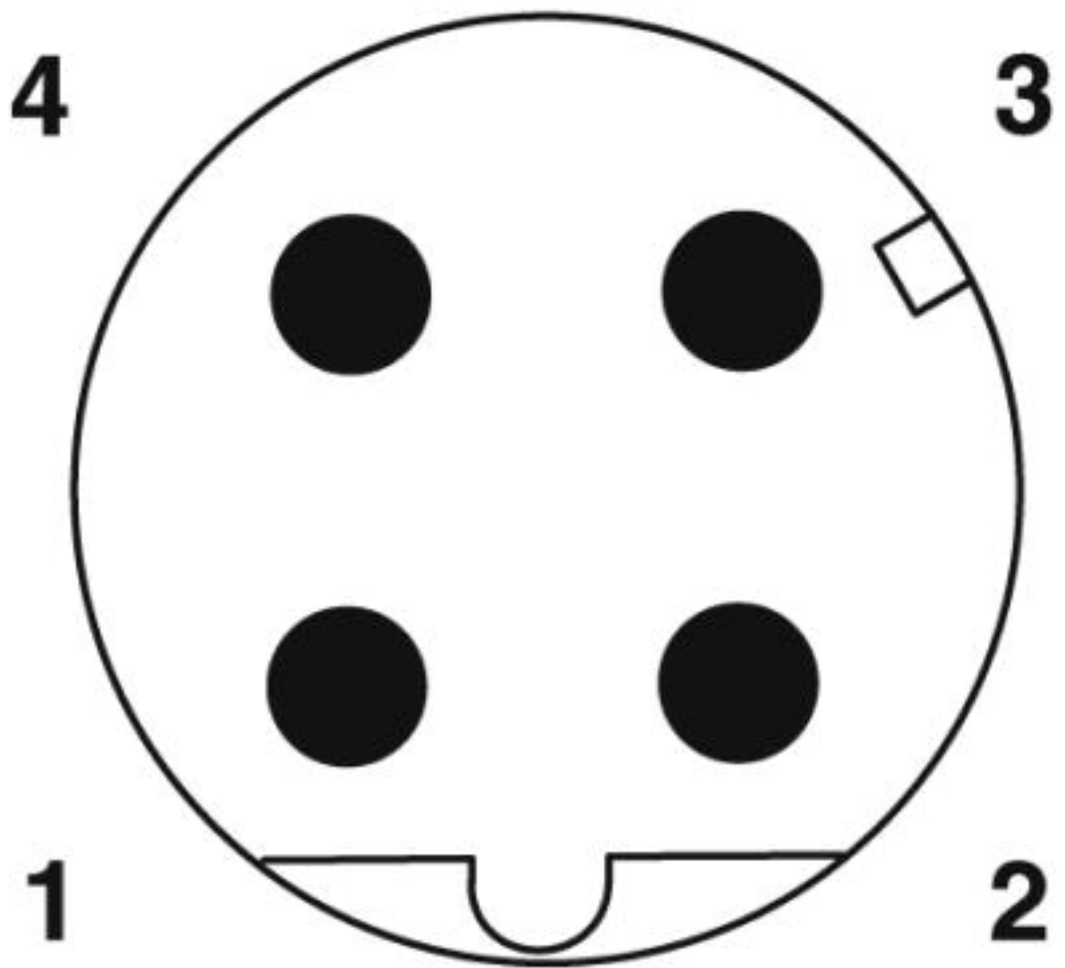
Schematic diagram
