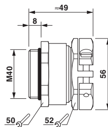
Dimensional drawing
