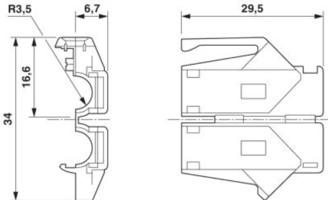
RJ45 bending protection sleeve
