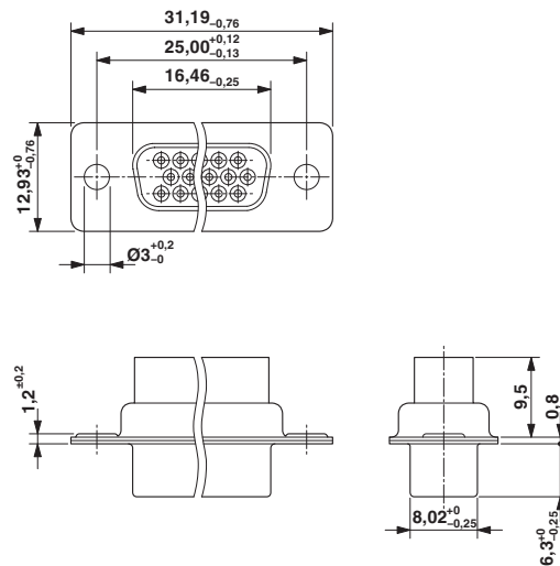
Dimensional drawing
