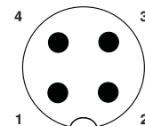
Pin assignment M12 plug, 4-pos., A-coded, view plug side
