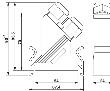
Dimensional drawing
