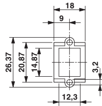
RJ45 panel mounting frame, IP20
