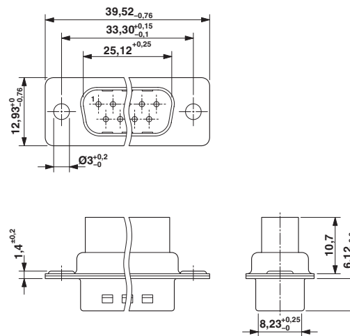
Dimensional drawing
