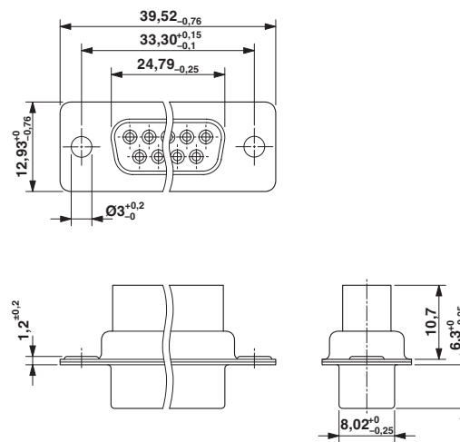
Dimensional drawing
