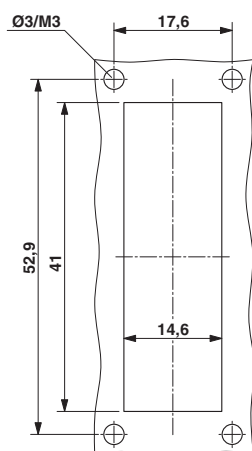
Dimensional drawing
