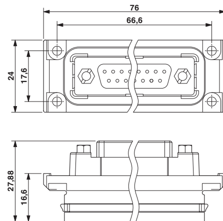
Dimensional drawing
