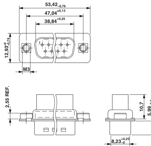
Dimensional drawing
