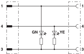
Contact assignment of M8 plugs / M12 sockets
