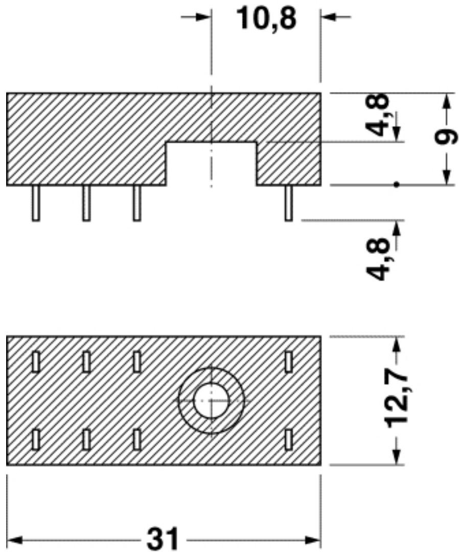
Dimensional drawing
