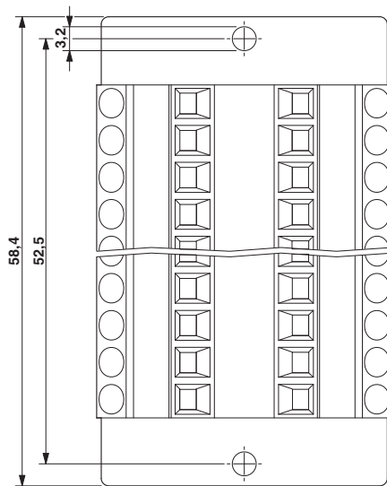
Dimensional drawing
