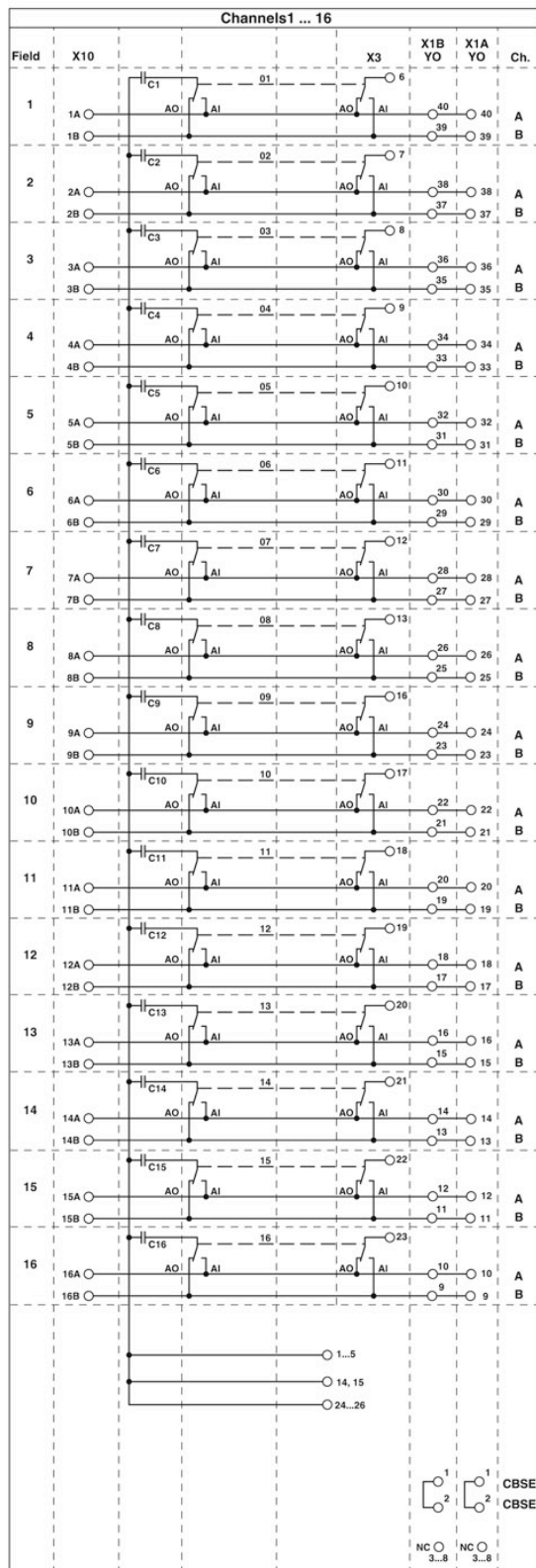
Circuit diagram
