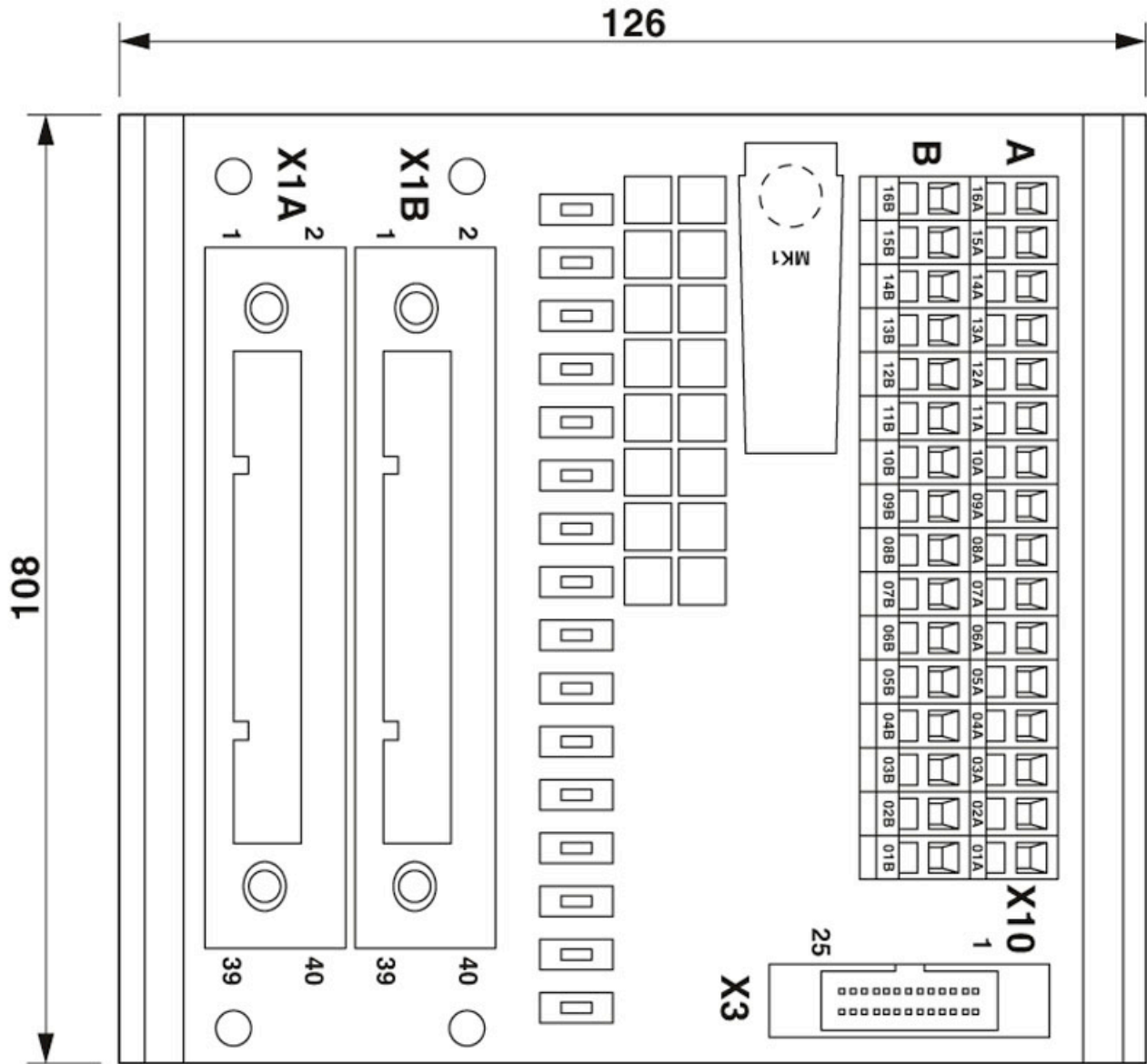
Dimensional drawing
