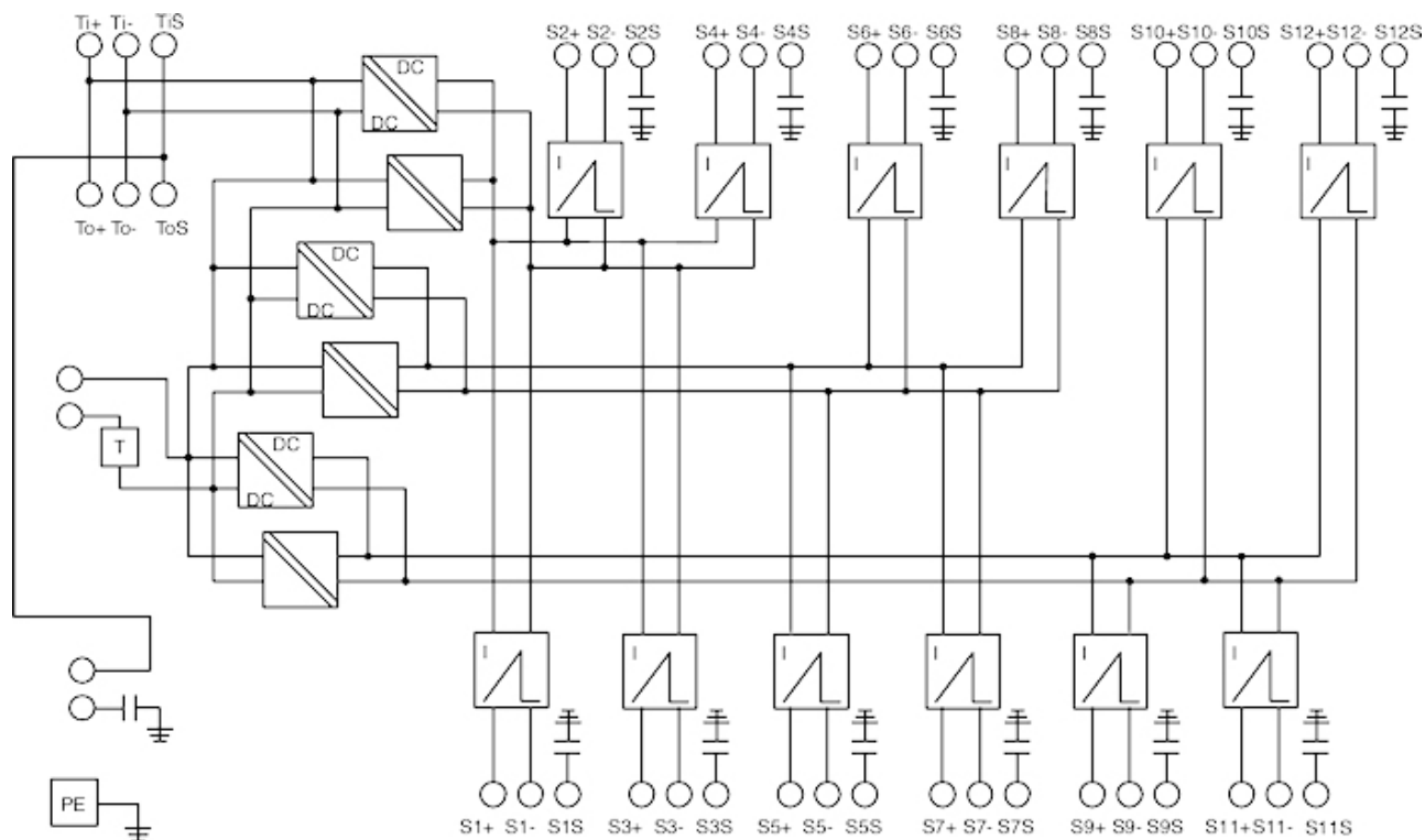
Block diagram
