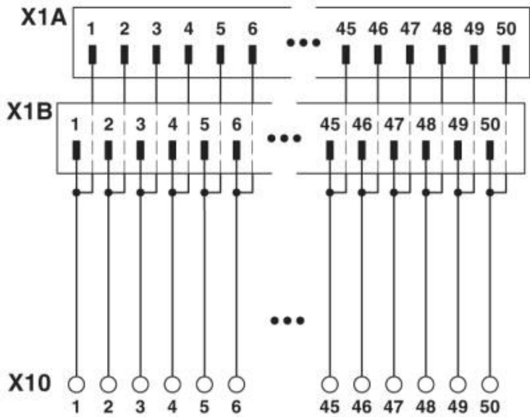
Circuit diagram
