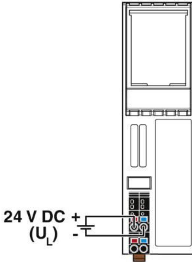
Connection diagram
