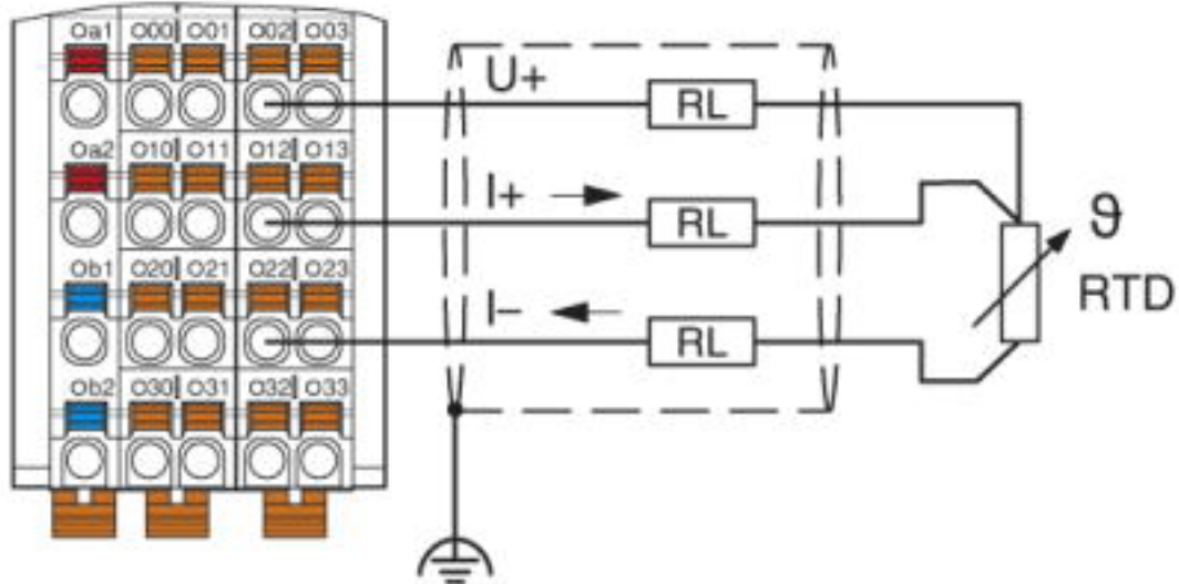
Connection example: 3-wire connection
