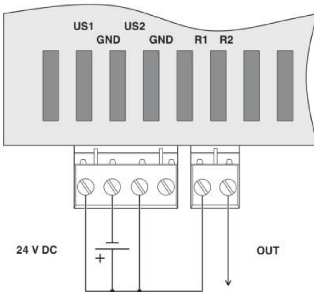
Connection diagram
