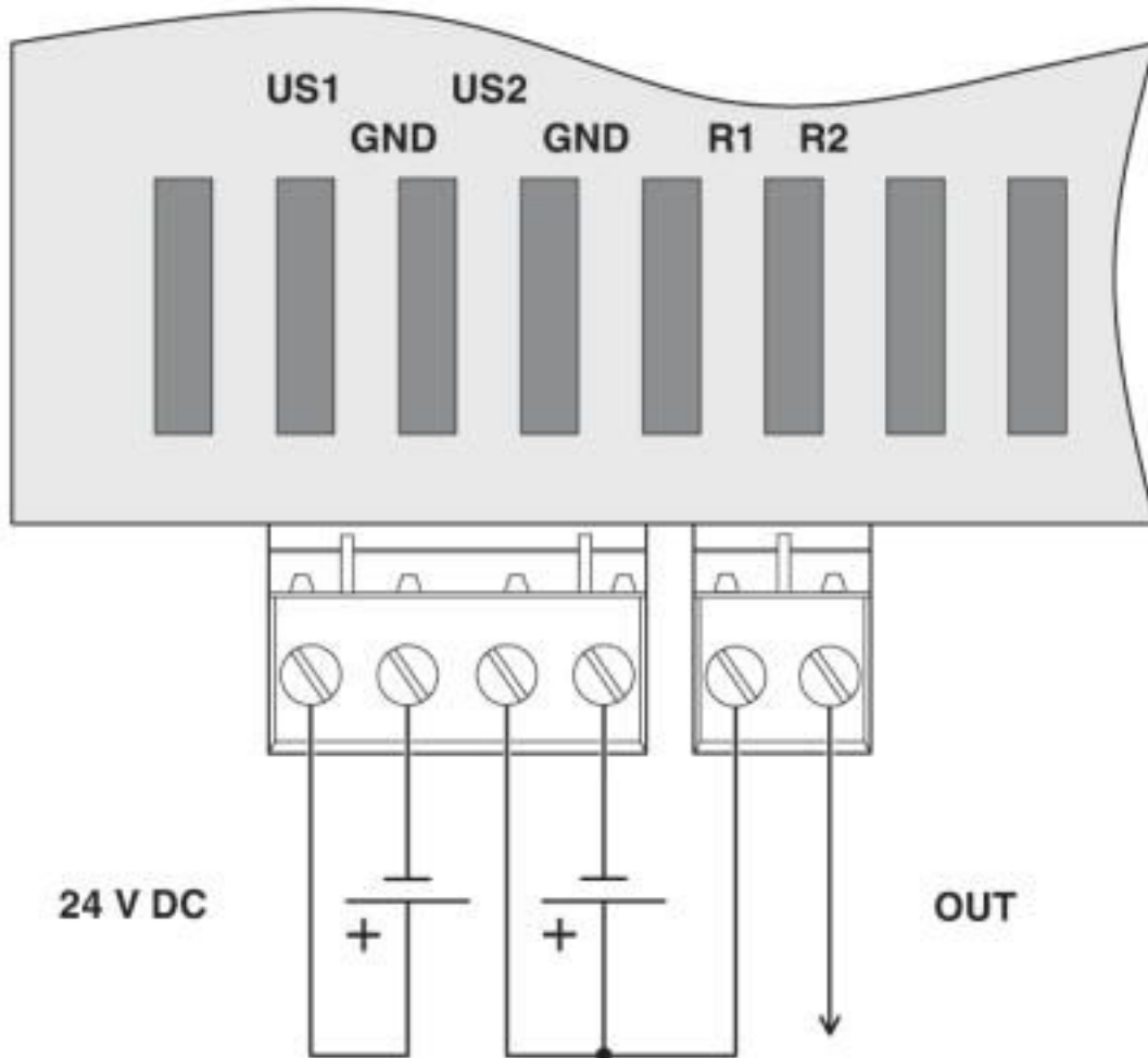
Connection diagram
