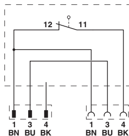
Circuit diagram
