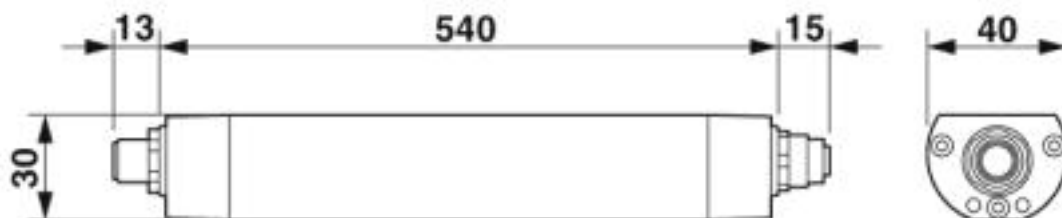
Dimensional drawing
