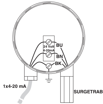
Application drawing
