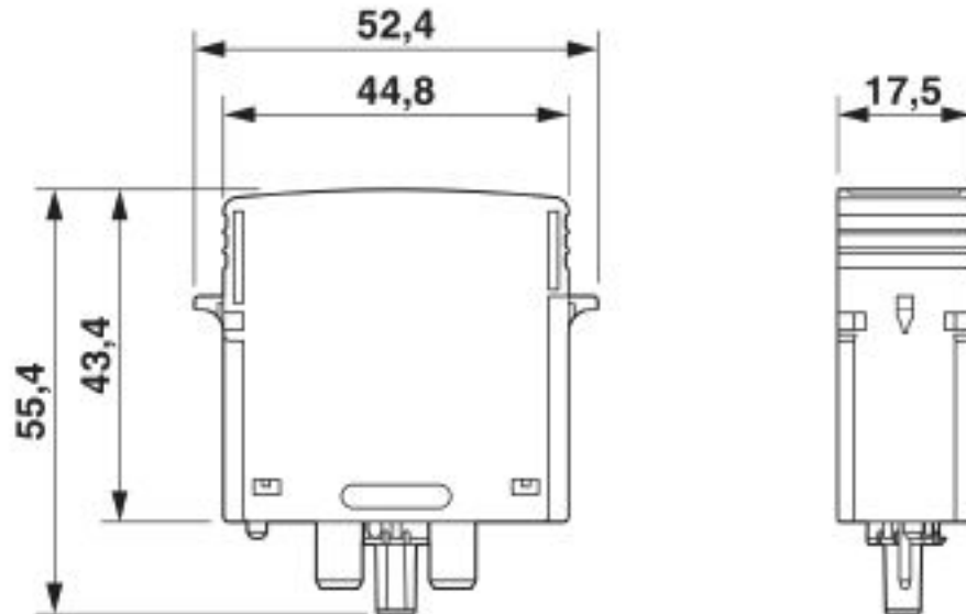
Dimensional drawing
