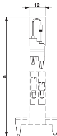
Dimensional drawing
