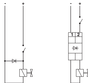
Circuit diagram
