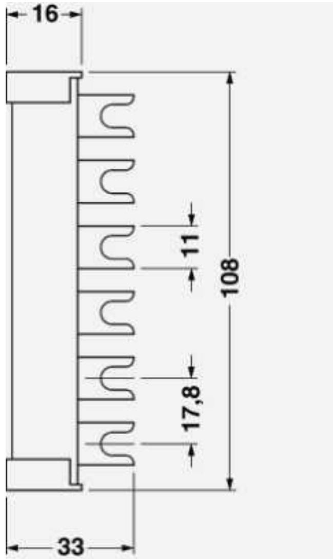
Dimensional drawing
