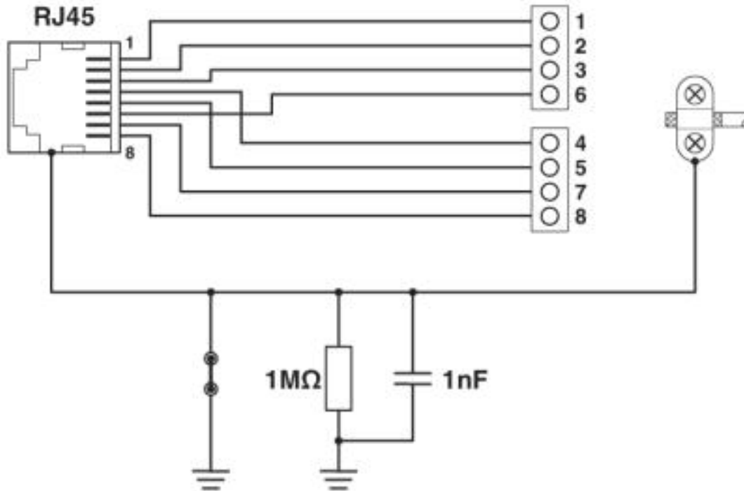
Circuit diagram
