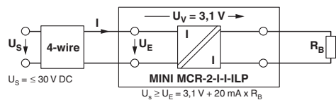
Application drawing
